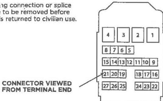
BCM Connector X6, Cavity 21
