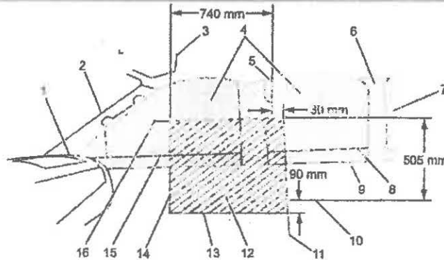
ROOF-RAIL MOUNTED HEAD-CURTAIN AIRBAG DEPLOYMENT ZONES - FRONT PASSENGER SIDE - DRIVER AND OUTBOARD FRONT SEAT FULLY LOWERED
