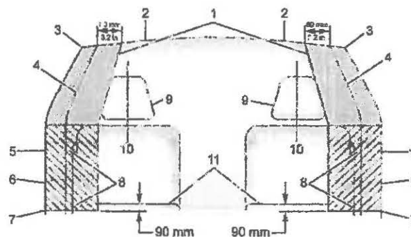
ROOF-RAIL MOUNTED HEAD CURTAIN AIRBAG - DRIVER AND OUTBOARD FRONT PASSENGER DEPLOYMENT ZONES - VIEW FROM REAR OF VEHICLE
