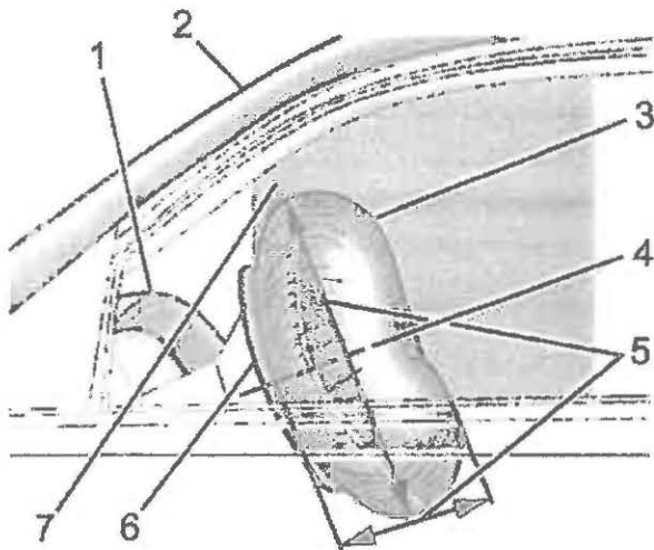
FRONT VIEW OF DRIVER INFLATED AIRBAG DEPLOYMENT ZONE
